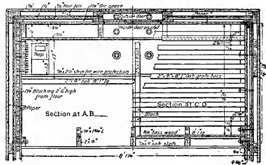
Fig. 282. Sectional Plan Showing Ice Box.
